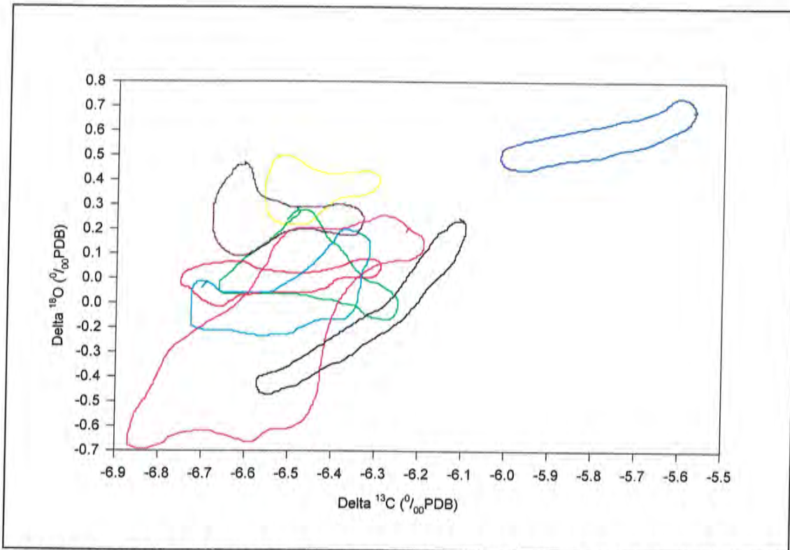
Figure 7.1. (a) Isotopic ratios of oxygen and carbon for otoliths samples of S. lemuru from Geraldton, Fremantle and Carnarvon. (b) Outlines of groupings from (a) for different regions and years.
