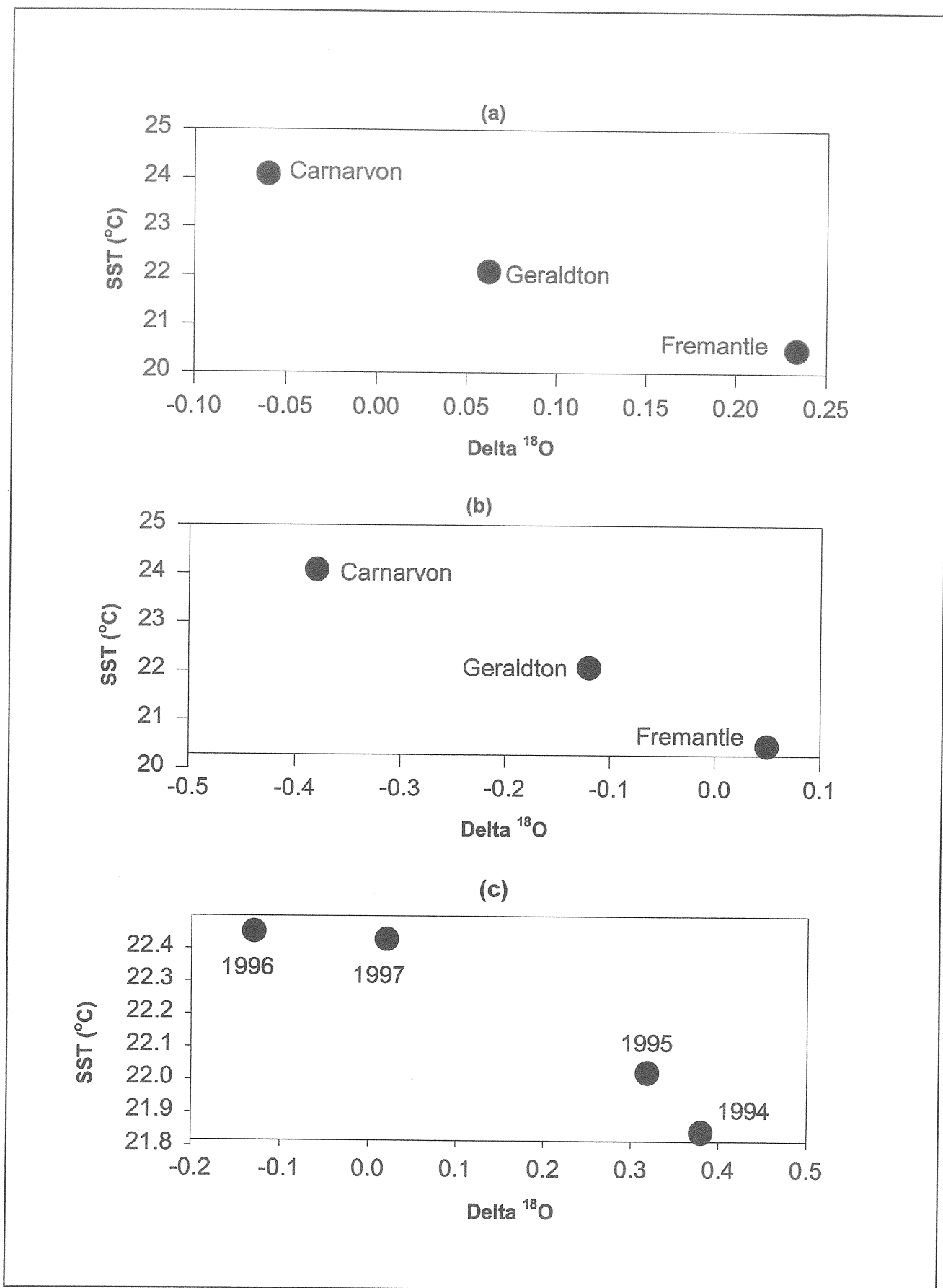
Figure 7.3. Relationship between SST and mean isotopic ratios of oxygen for (a) all samples of S. lemuru otoliths from Geraldton, Fremantle and Carnarvon, and (b) for a similar sized S. lemuru otoliths obtained within a four month period in 1997 at the same regions, and (c) samples of S. lemuru from Geraldton between 1994 and 1997.
