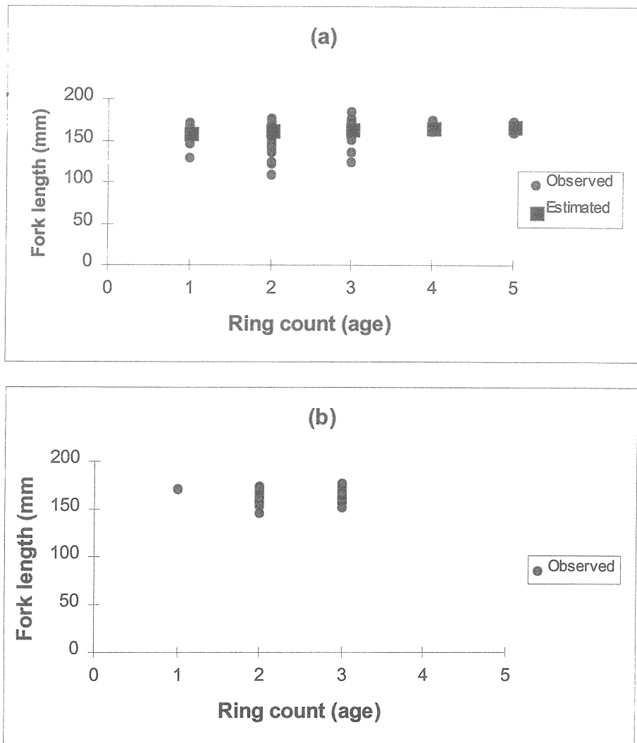
Figure 6.3. (a) von Bertalanffy curve for S. lemuru based on counts of rings on scales which included discrepancies between successive counts. (b) Length versus age, with age estimated using only counts for which there were zero discrepancies.
