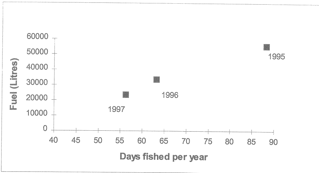
Figure 8.9. Relationship between fuel used and days fished for the 24 m vessel annually from 1995 to 1997, using the fuel data from Fisheries WA’s compulsory catch and effort reporting system.
