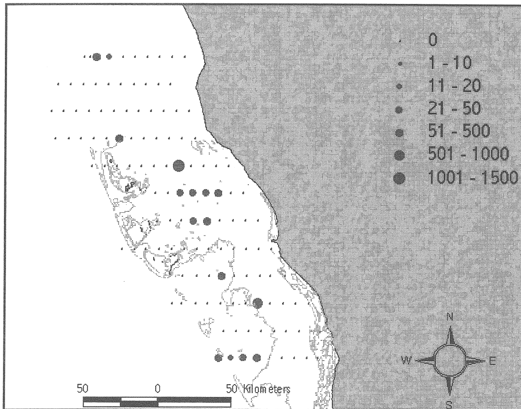
Figure 9.5. Concentrations of S. lemuru eggs (number 100\text{ m}^{-3} ) expressed using a relative scale for the plankton survey conducted between Kalbarri and Dongara in February 1997. Spawning area = 2308\text{ km}^2 .
