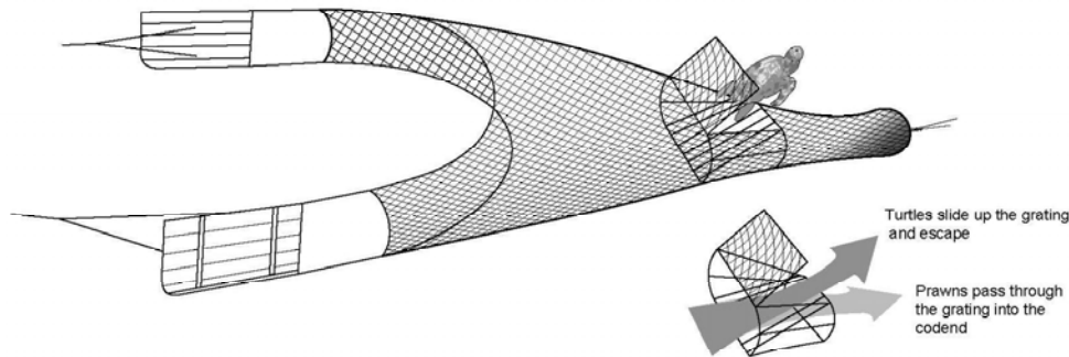
Figure 1 Diagram of one style of TED.
