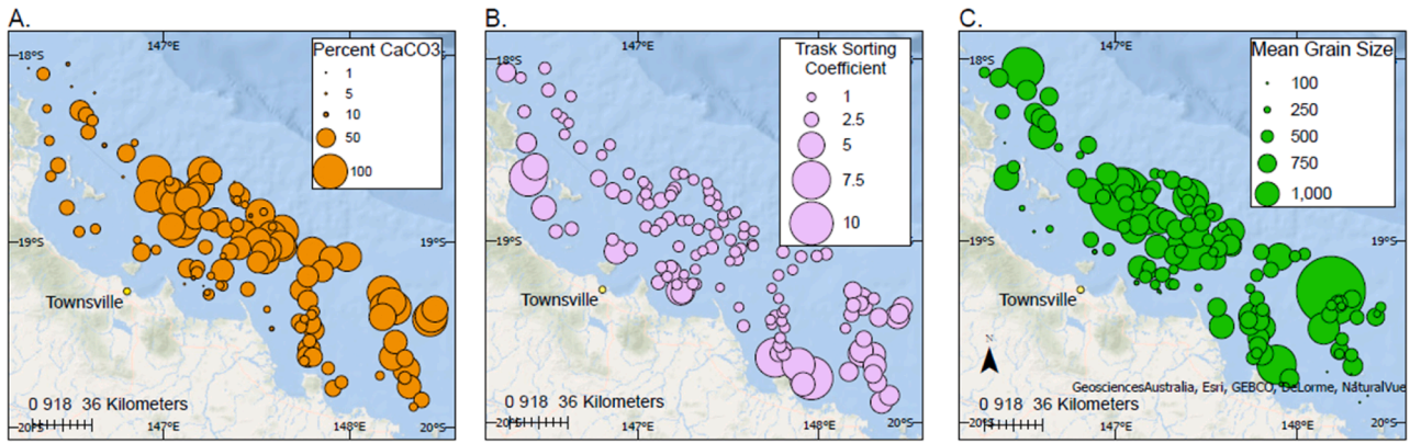
Fig. 2. Map of sediment parameter results by site from the survey off Townsville. A) percent calcium carbonate content, B) sediment sorting value measured in Trask units ( \emptyset ), larger bubbles mean more poorly sorted, C) mean grain sizes in microns.
